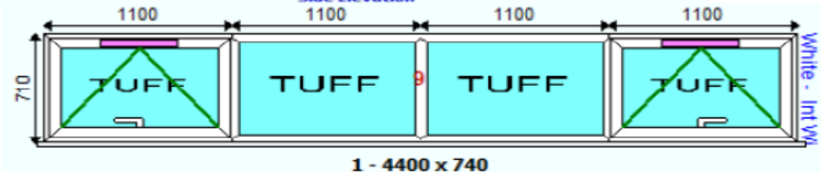
Side Elevation
